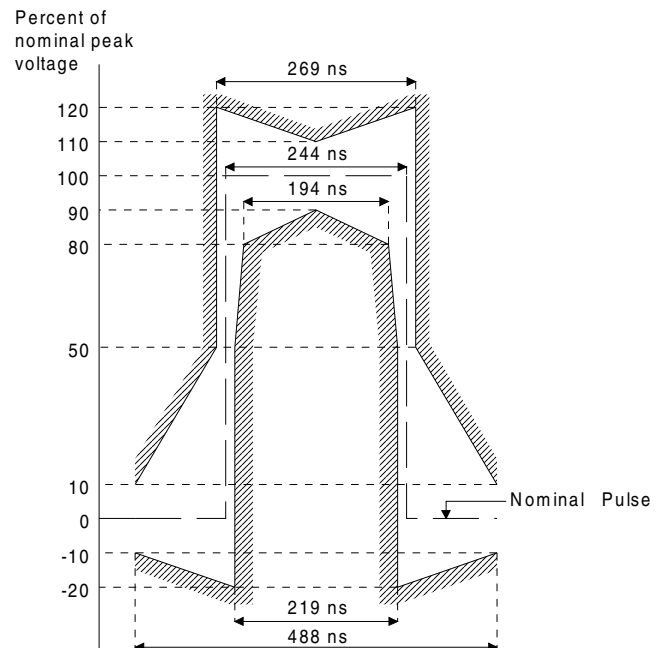
Figure 7. Pulse Mask at E1 Interface
