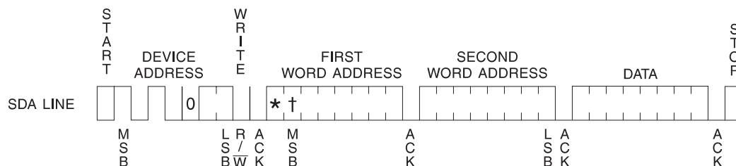
Figure 2. Byte Write
