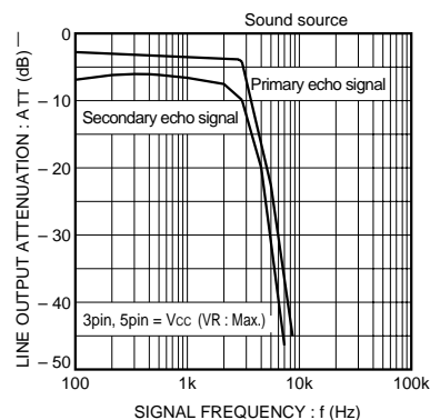
Echo signal frequency characteristics
