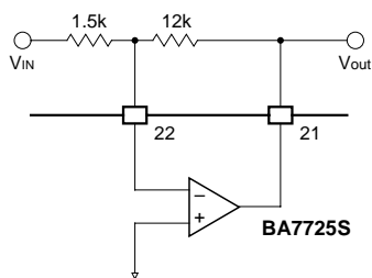
Microphone amplifier frequency characteristic measurement circuit Fig.2
