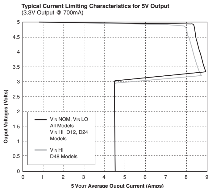
Figure 2b. Current Limiting Characteristics for 5V Output
