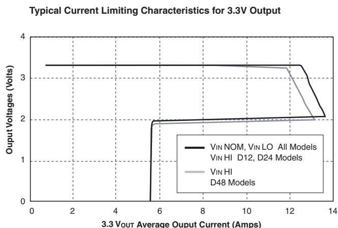
Figure 2a. Current Limiting Characteristics for 3.3V Output
