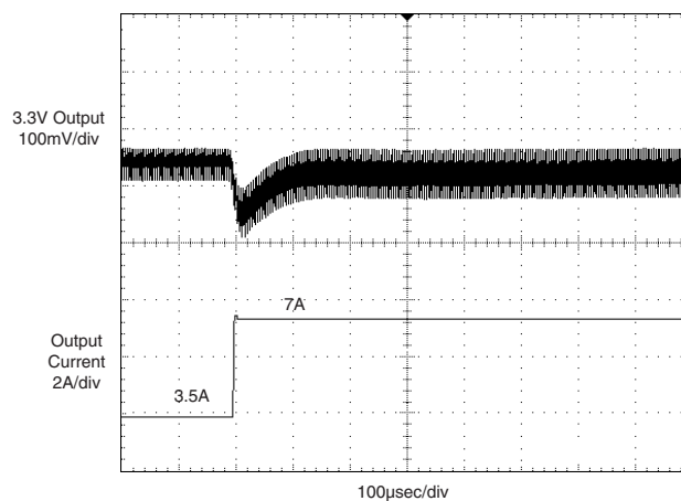
3.3V Output Half-Load to Full-Load Transient Response (VIN = nominal, 5V @ 600mA, external 1μF output capacitors.)
