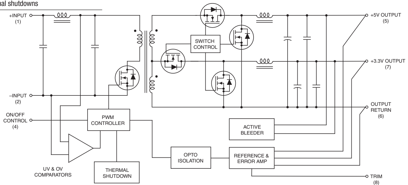
Figure 1. Simplified Schematic
