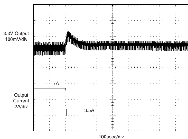
3.3V Output Full-Load to Half-Load Transient Response (VIN = nominal, 5V @ 600mA, external 1μF output capacitors.)
