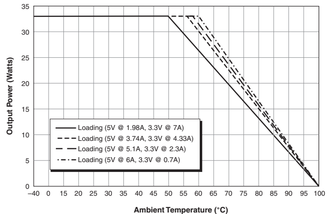
Output Power vs. Ambient Temperature V_{IN} = 36V , Natural Convection Air flow
