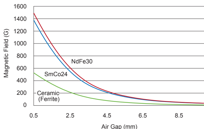
Figure 51: Magnetic Field versus Air Gap for a magnet 6 mm in diameter and 2.5 mm thick.
