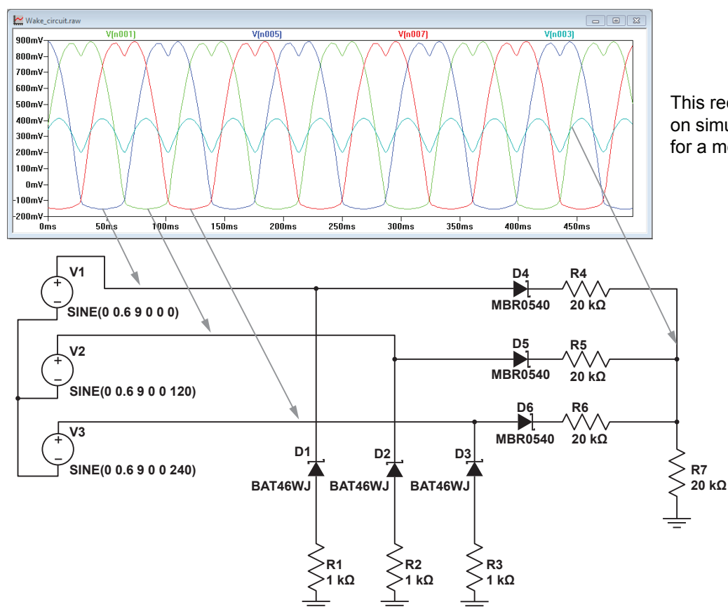
Figure 30: SPICE Simulation Example for Filtered BEMF Signal
