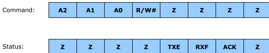
Figure 6.7 SPI Command and Status Structure
