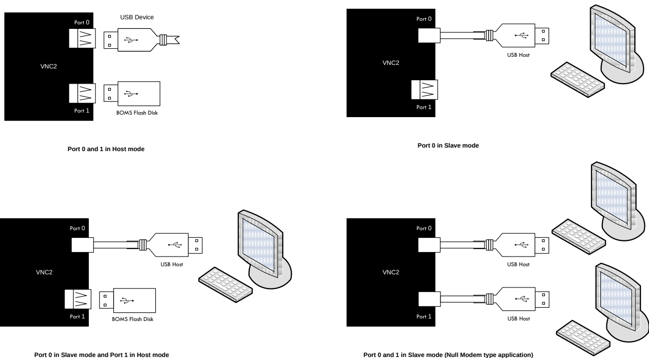
Figure 7.1 USB Modes
