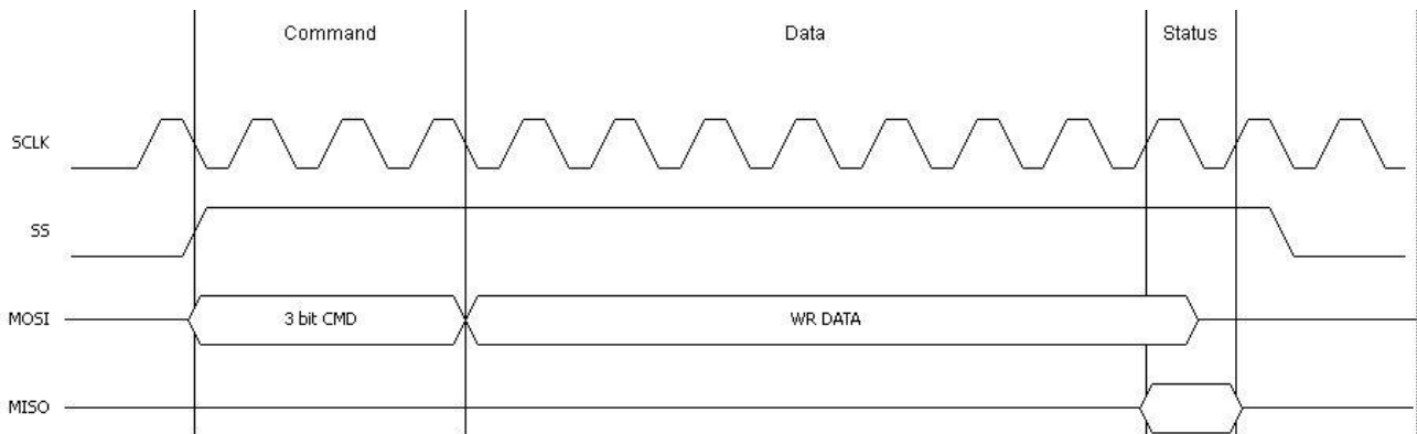
Figure 6.13 VNC1L Mode Data Write
