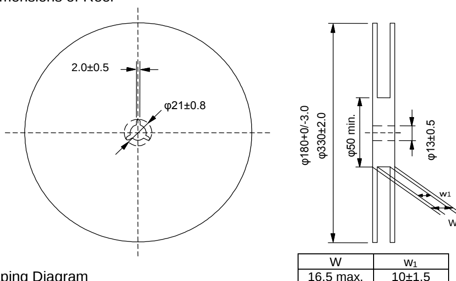
Fig.2 Dimensions of Reel
