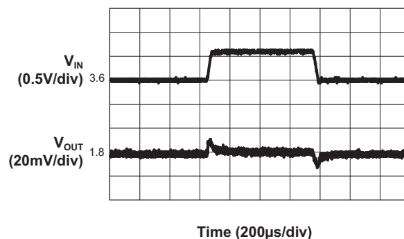
Line Transient
