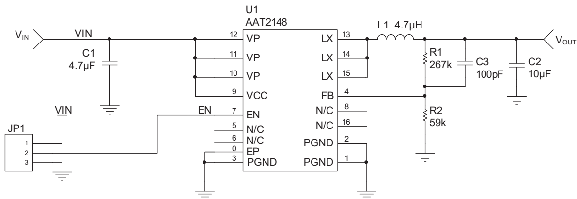
Figure 4: AAT2148 Evaluation Board Schematic.
