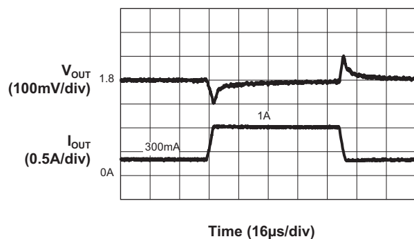
Load Transient
