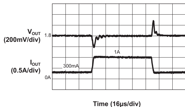
Load Transient
