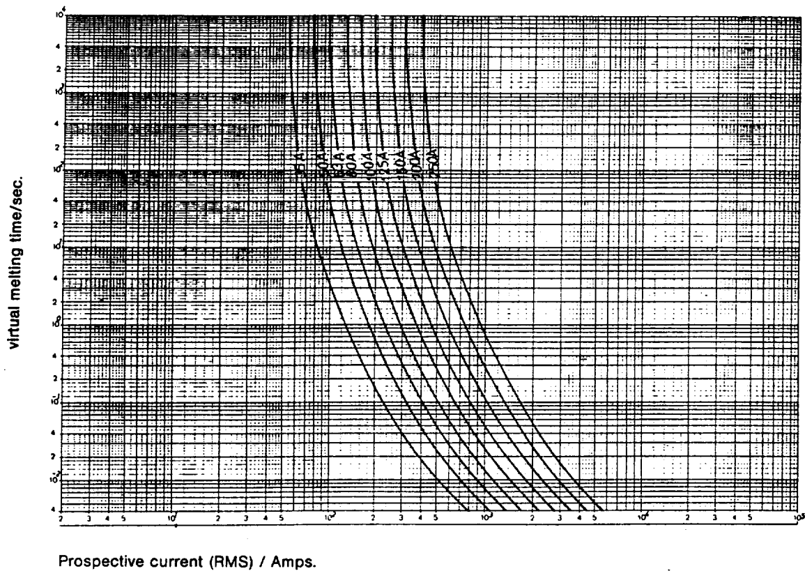
Medium Time current characteristic
