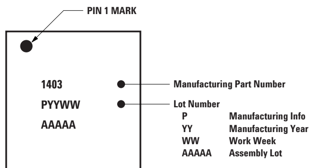
Figure 9. Marking specifications
