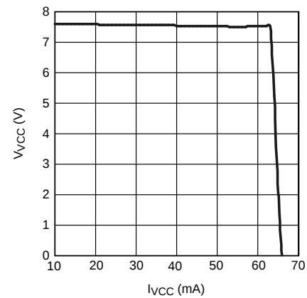
Figure 2. V_{CC} vs I_{VCC}
