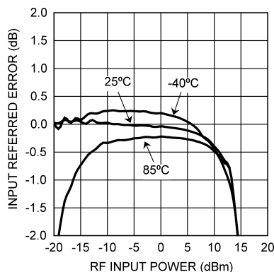
Figure 23. Input referred Error vs. RF Input Power
