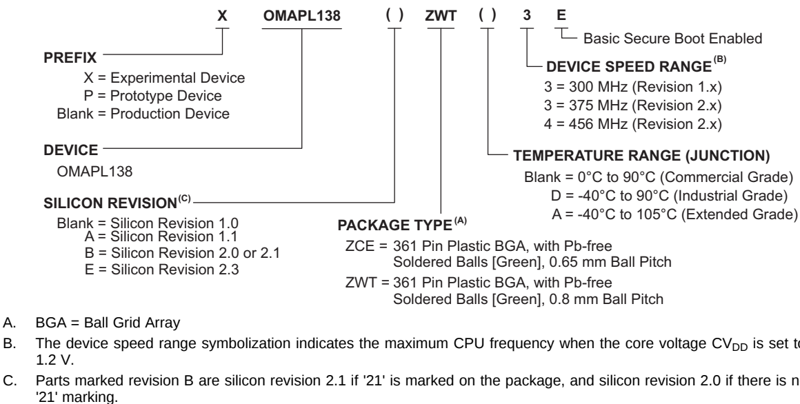
Figure 7-1. Device Nomenclature
