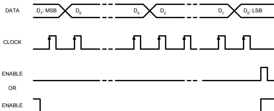
Figure 17: Serial Data Input Timing
