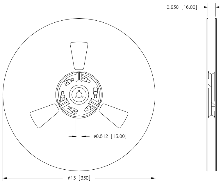
Figure 21: Reel Dimensions
