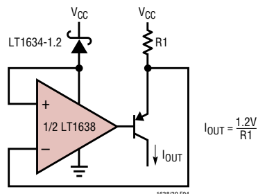
Figure 4. Current Source
