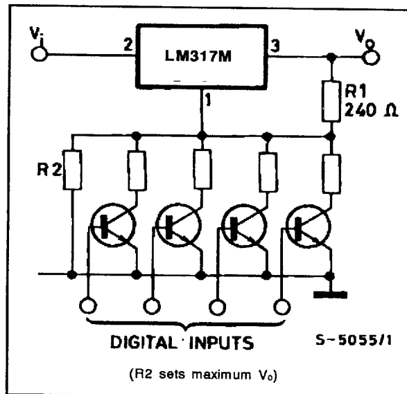
Digitally Selected Outputs.
