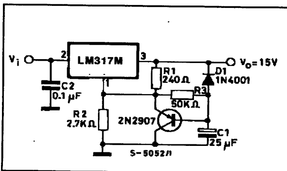
Slow Turn-on 15V Regulator.
