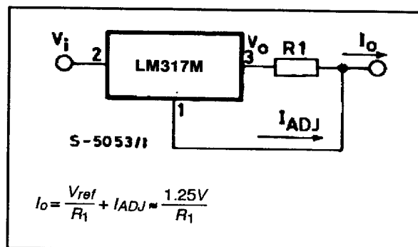
Current Regulator.
