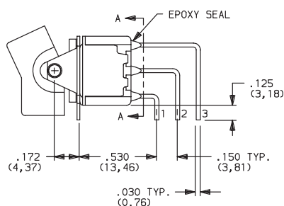
.050 TYP. (1, 27) TERM. WIDTH
