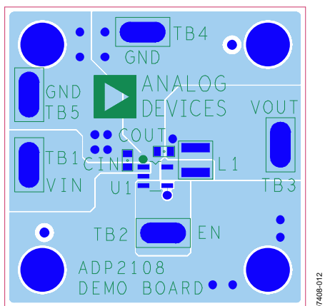
Figure 11. Top Layer, Recommended Layout for TSOT
