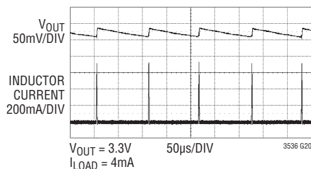
Output Voltage Ripple in Burst Mode Operation
