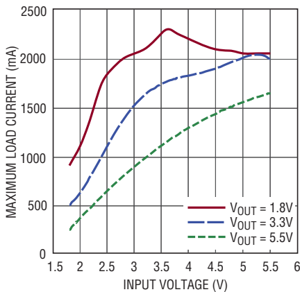
Maximum Load Current in PWM Mode vs Input Voltage 1MHz Switching Frequency, 4.7 \mu\text{H} Inductor Value
