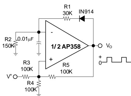
Pulse Generator
