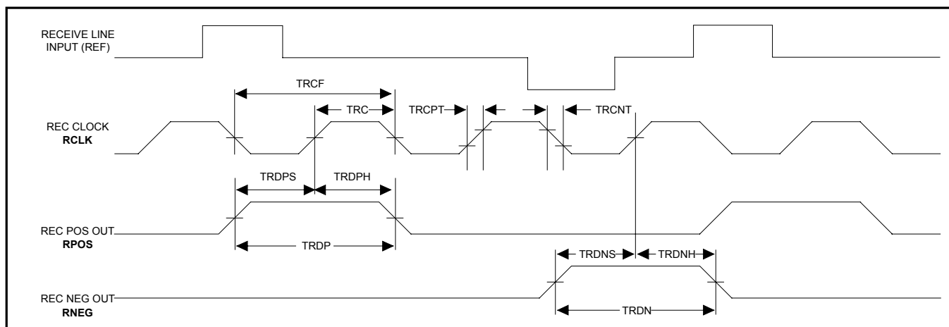
FIGURE 2: Receive Waveforms
