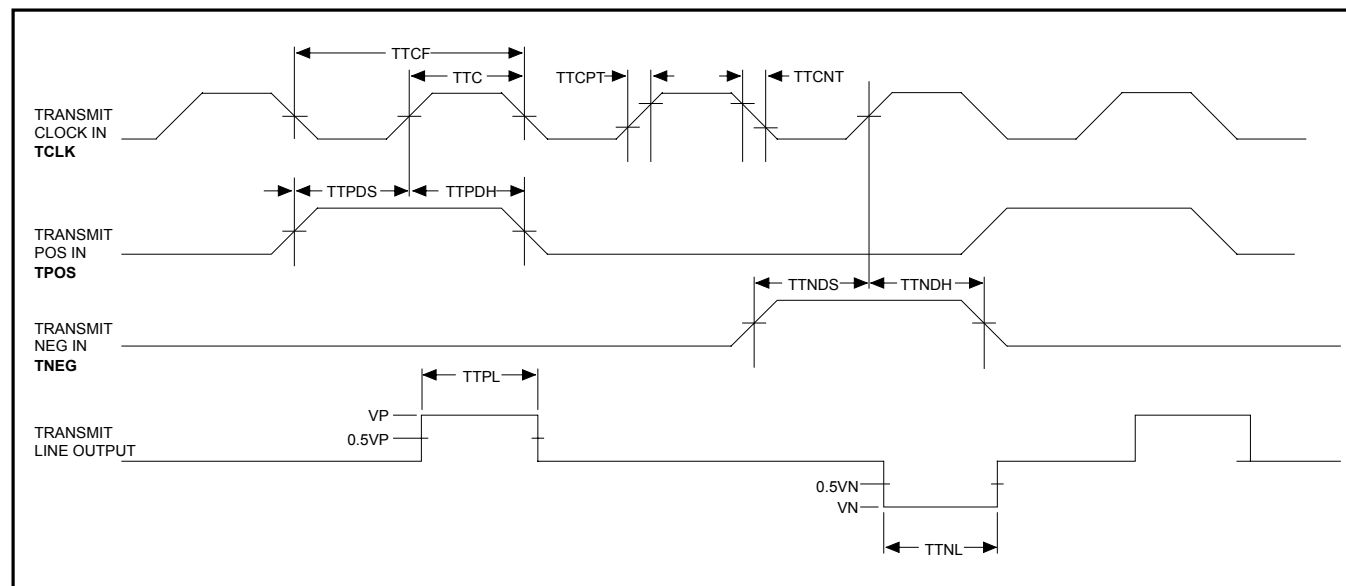
FIGURE 3: Transmit Waveforms
