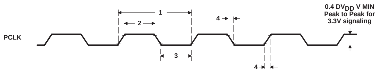
Figure 47. PCLK Timing
