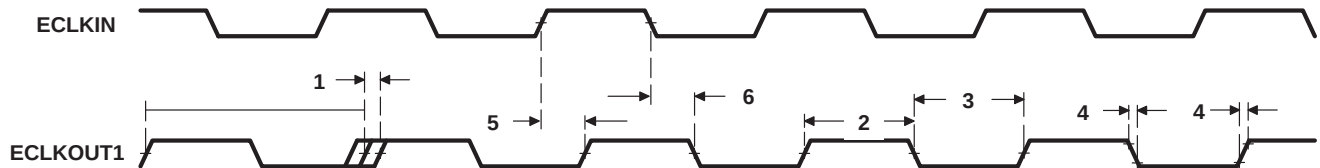
Figure 20. ECLKOUT1 Timing
