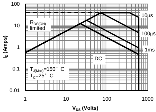
Figure 9: Maximum Forward Biased Safe Operating Area for AOB11N60 (Note F)
