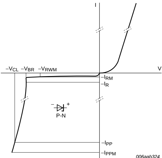
Fig 4. V-I characteristics for a bidirectional ESD protection diode
