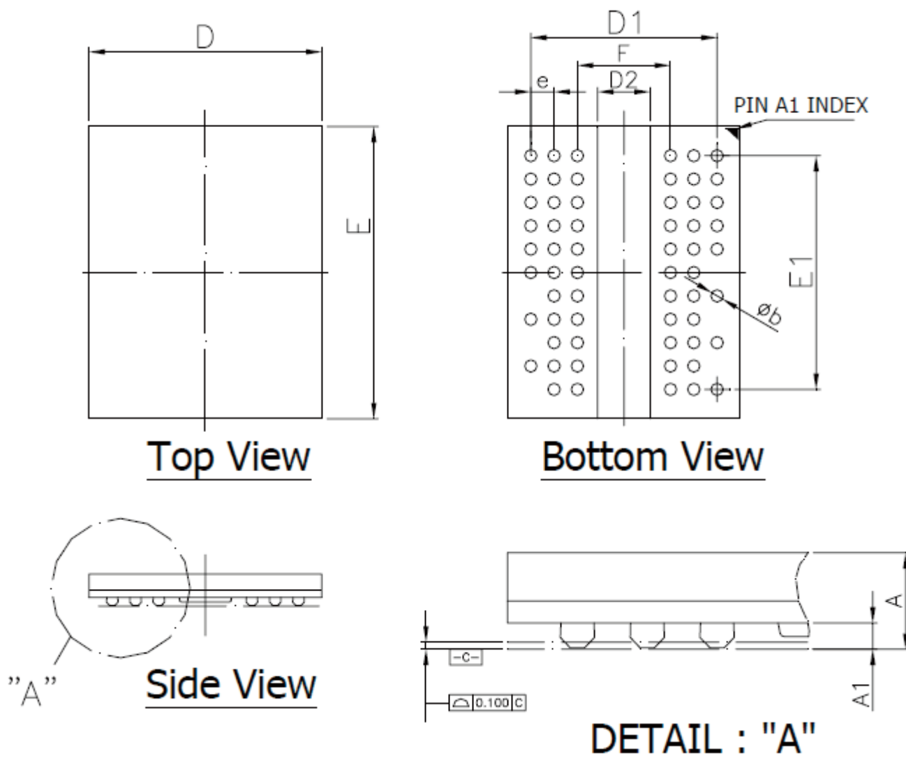
Figure 61. 60-Ball FBGA 8x10x1.2mm(max) Package Outline Drawing Information
