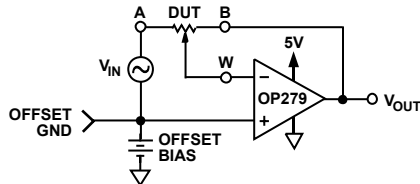
Figure 49. Test Circuit for Inverting Gain
