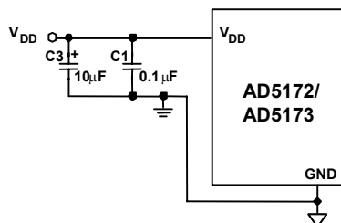
Figure 35. Power Supply Bypassing
