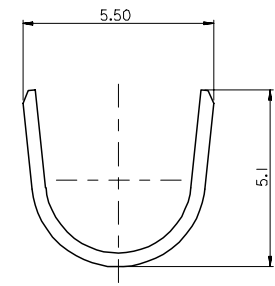
SECT. B-B
