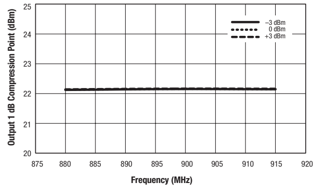
Figure 18. Mixer B OP1dB vs Frequency and LO Power
