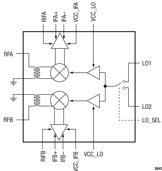
Figure 1. SKY73020 Block Diagram
