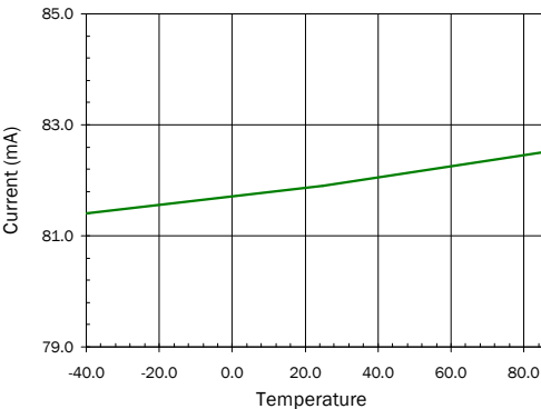
Id vs. Temperature (Bias Tees)
