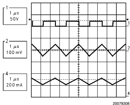
Operational Waveforms
