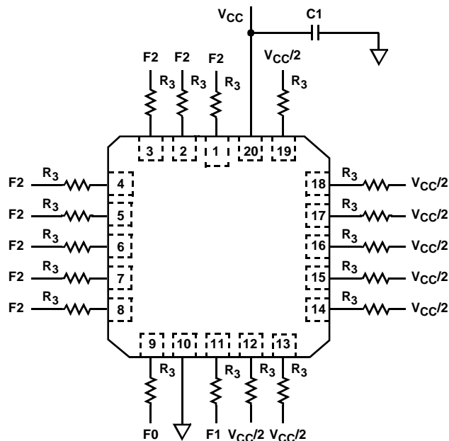
MR82C82 CLCC
