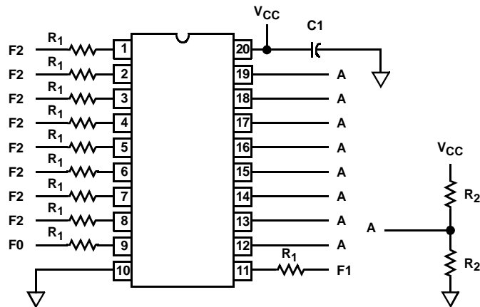
MR82C82 CLCC
