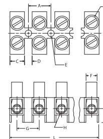
Dimensions mm
