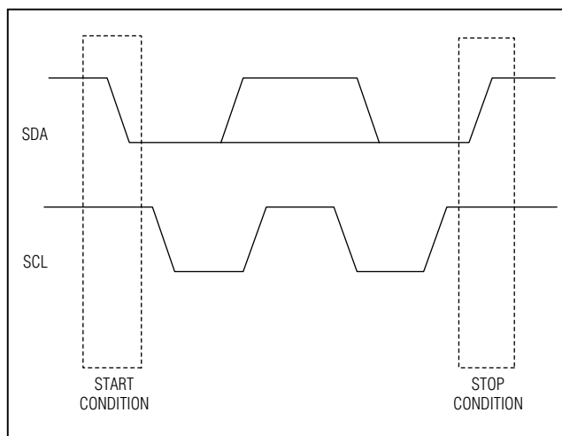
Figure 13. START and STOP Conditions
