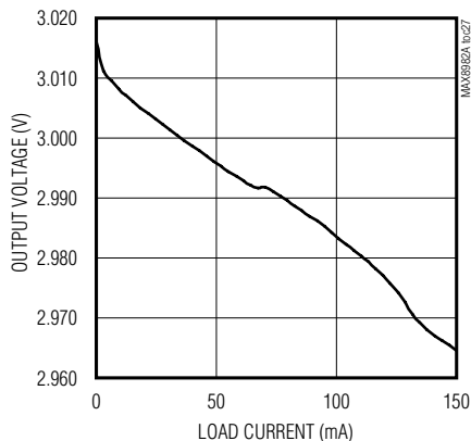
LD05 LOAD REGULATION
