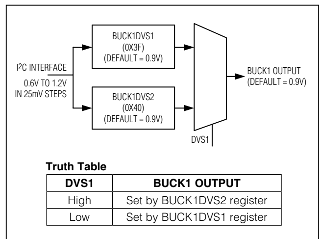
Figure 7. DVS1 Logic Diagram
