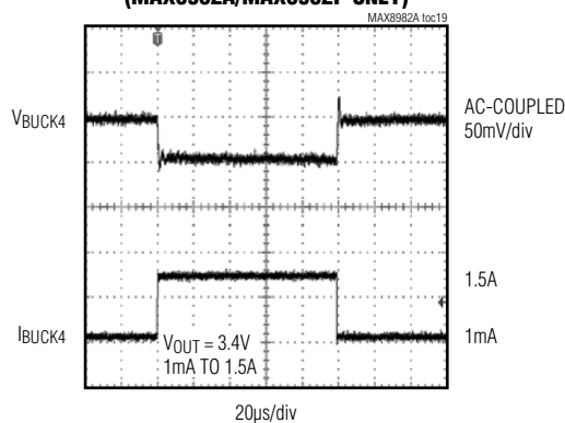
BUCK4 LOAD TRANSIENT (MAX8982A/MAX8982P ONLY)
