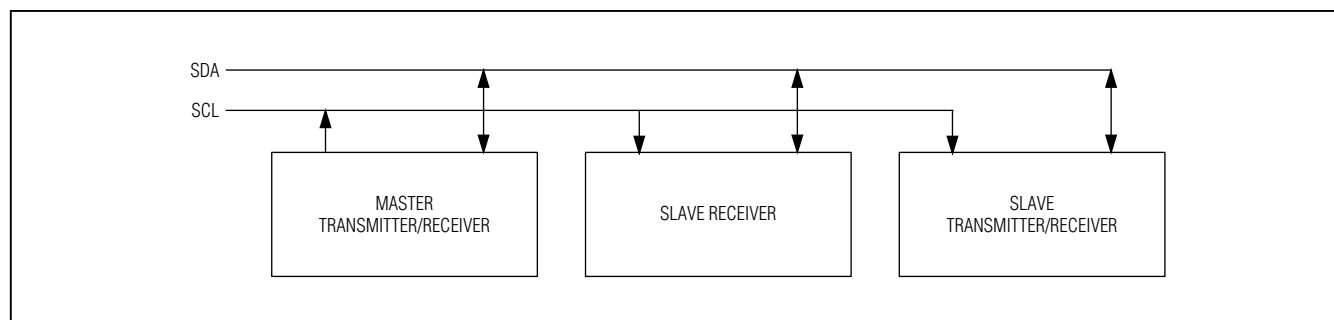
Figure 14. Master/Slave Configuration
