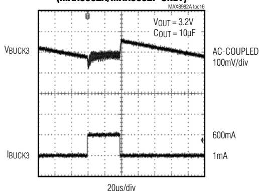
BUCK3 LOAD TRANSIENT (MAX8982A/MAX8982P ONLY)
