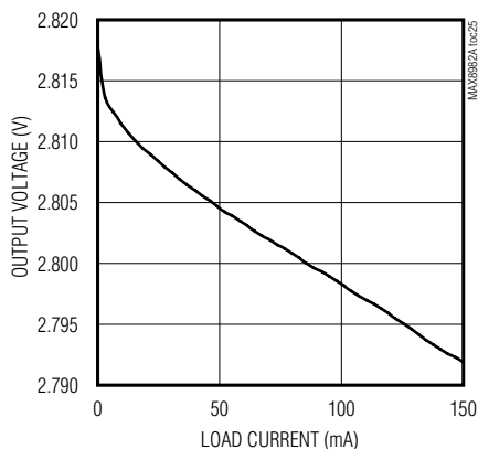
LD03 LOAD REGULATION
