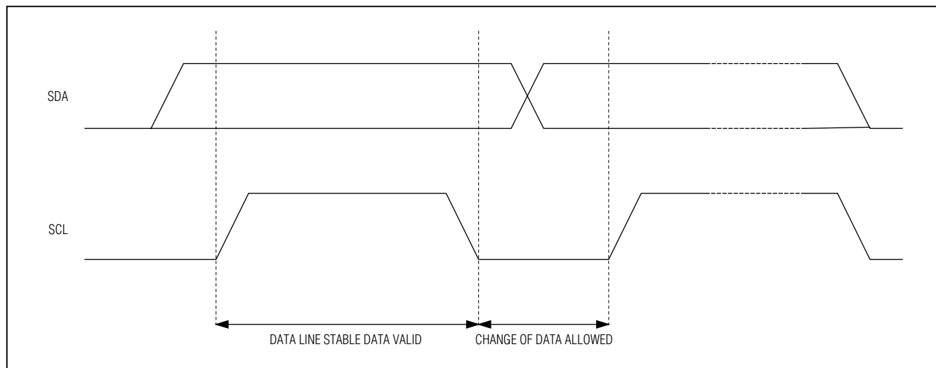
Figure 12. I 2 C Bit Transfer
