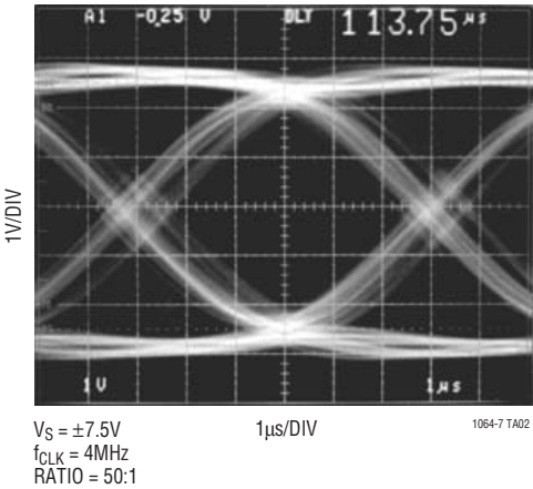
Eye Diagram
