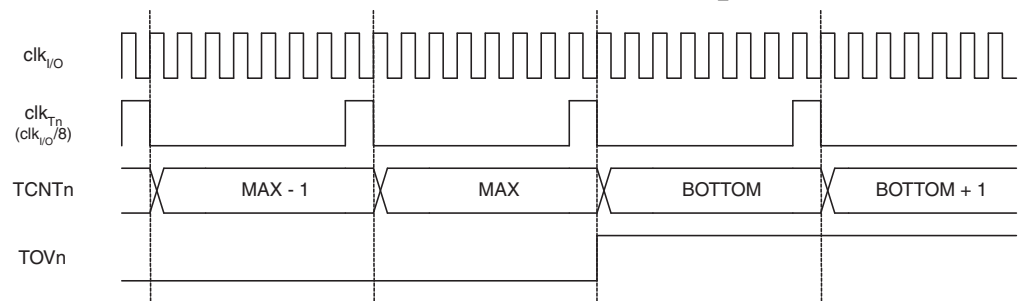
Figure 12-9. Timer/Counter Timing Diagram, with Prescaler ( f_{\text{clk\_I/O}}/8 )
