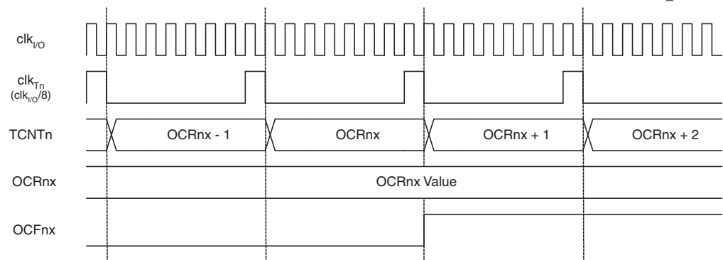
Figure 12-10. Timer/Counter Timing Diagram, Setting of OCF0x, with Prescaler ( f_{\text{clk\_I/O}}/8 )
