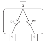
BAT68-06 BAT68-06W
