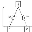
BAT68-05 BAT68-05W
