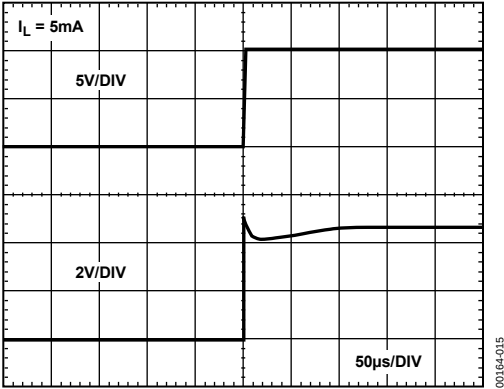
Figure 15. Turn-On Time
