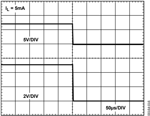
Figure 16. Turn-Off Time
