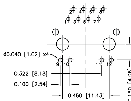
Recommended PCB Layout (Component Side)
