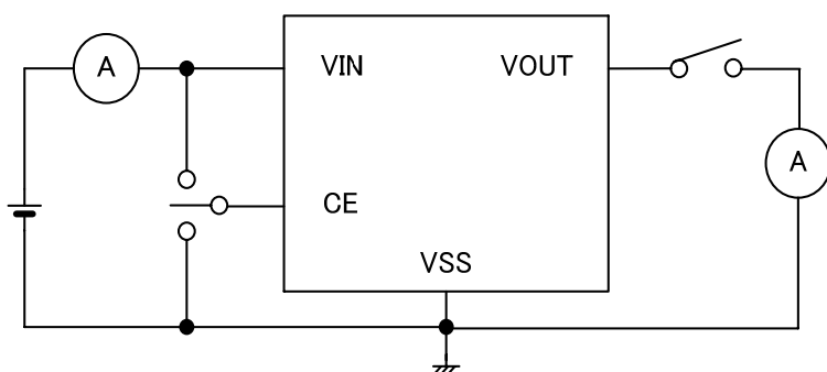
Circuit ③
