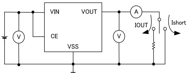
Circuit ②
