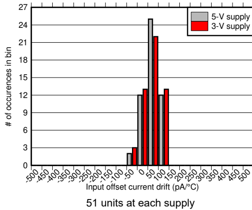
Figure 6-49. Input Offset Current Drift Distribution
