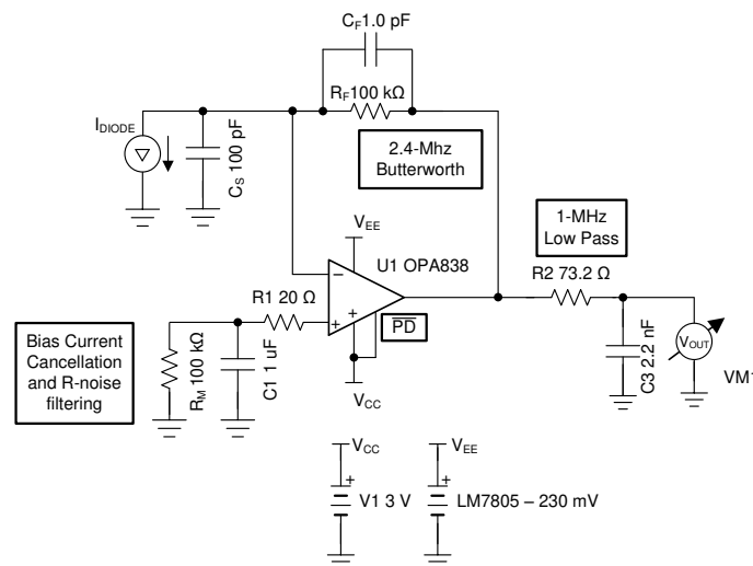
Figure 8-7. 100-k \Omega Wide Bandwidth Transimpedance Design
