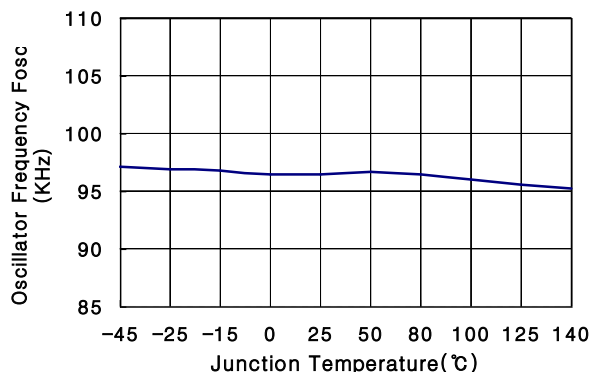
Figure 7. Oscillator Frequency
