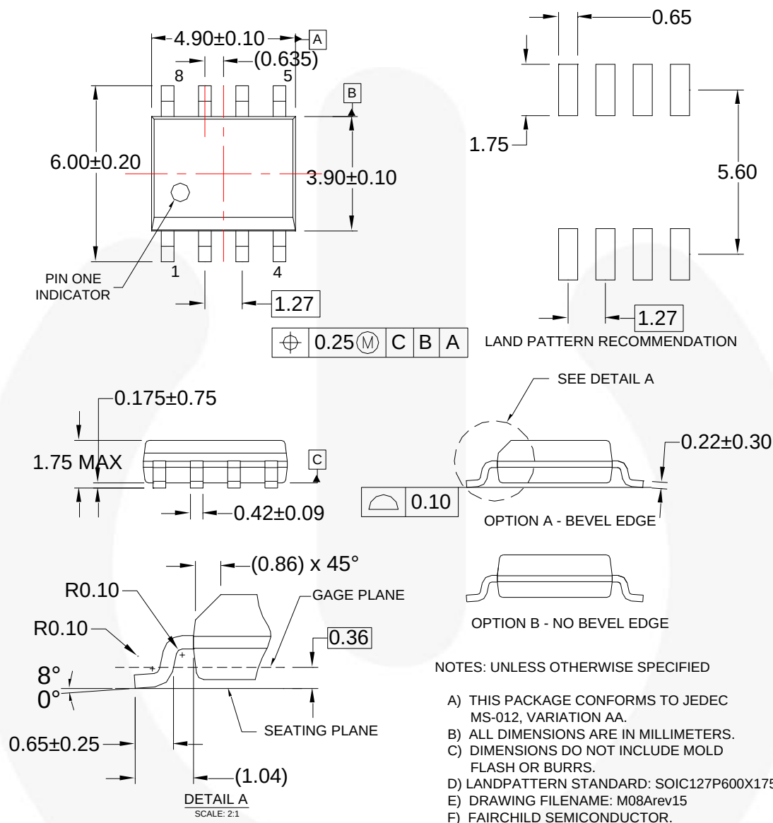
Figure 16. 8-Lead, Small Outline Package (SOP)
