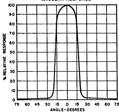
ANGULAR RESPONSE
