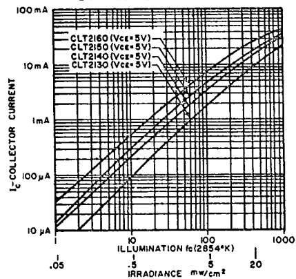
LIGHT CURRENT vs. IRRADIATION
