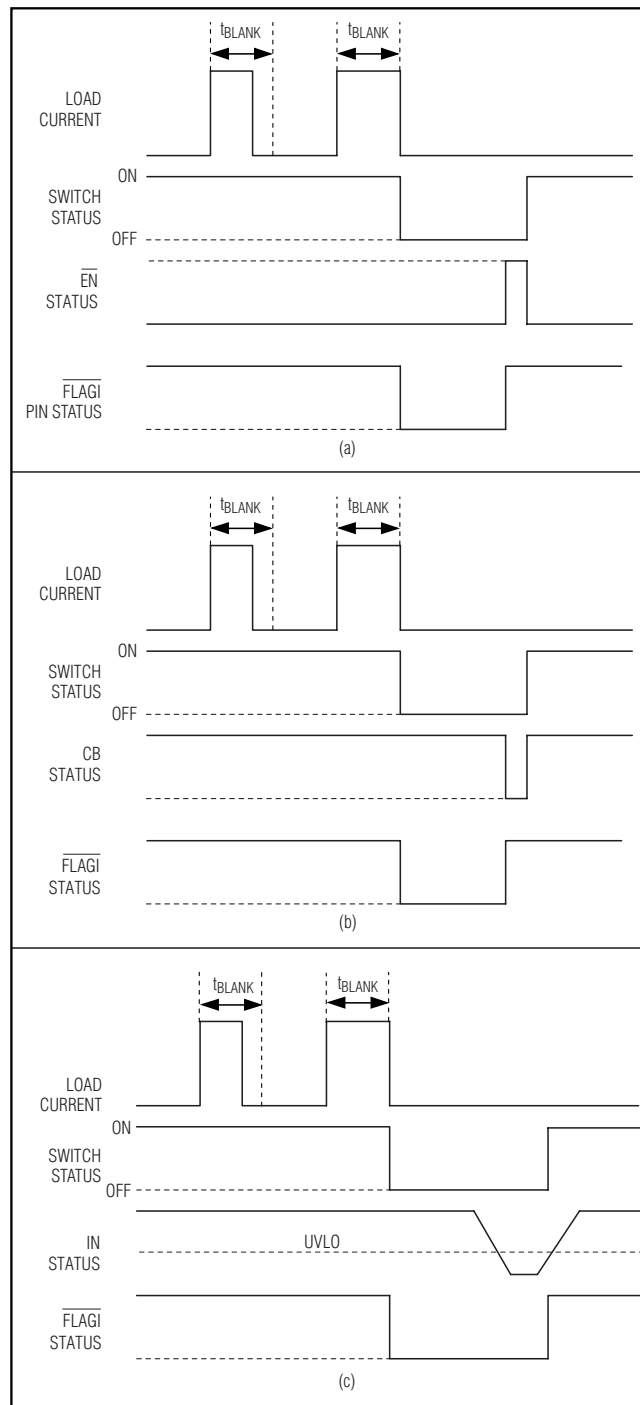
Figure 6. Latchoff Fault Blanking (MAX4881/MAX4882/MAX4883B/MAX4884B/MAX4893B)
