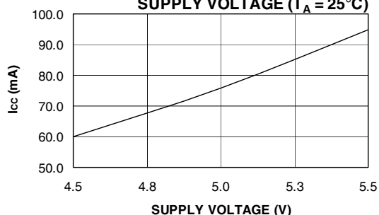
STAND-BY I_{CC} VS. SUPPLY VOLTAGE ( T_A = 25^\circ C )
