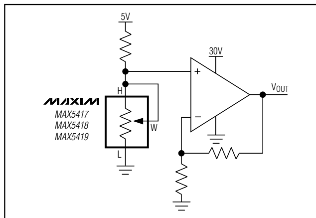
Figure 10. Positive LCD Bias Control Using a Variable Resistor
