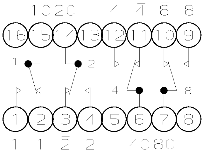
SCHEMATIC (POSITION 0)
