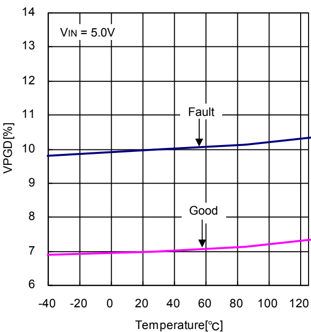
Figure 17. PGD Voltage vs Temperature
