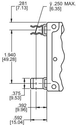
Clip Terminal
