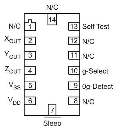
Figure 1. Pin Connections
