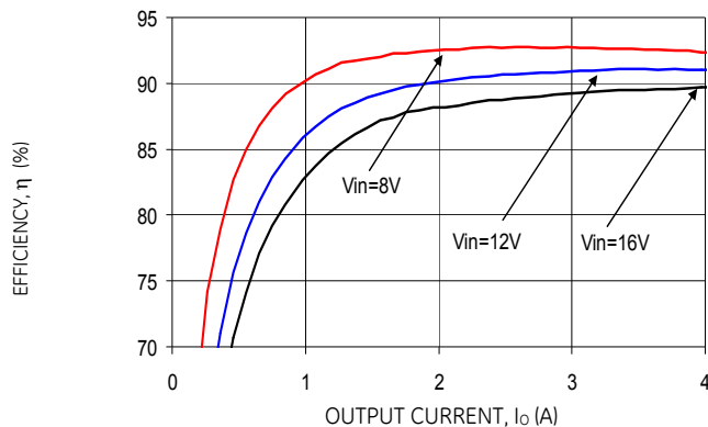
Figure 25. Converter Efficiency versus Output Current.
