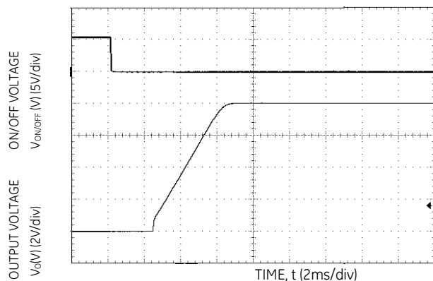
Figure 47. Typical Start-up Using On/Off Voltage ( I_o = I_{o,max} ).
