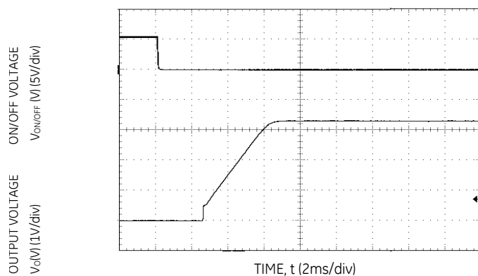
Figure 29. Typical Start-up Using On/Off Voltage ( I_o = I_{o,max} ).
