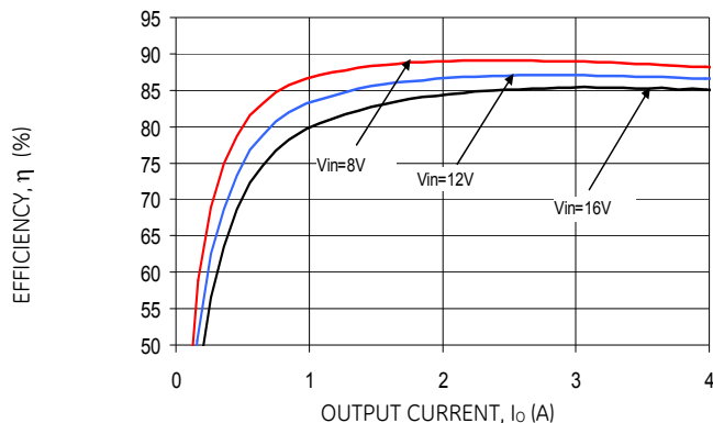
Figure 13. Converter Efficiency versus Output Current.
