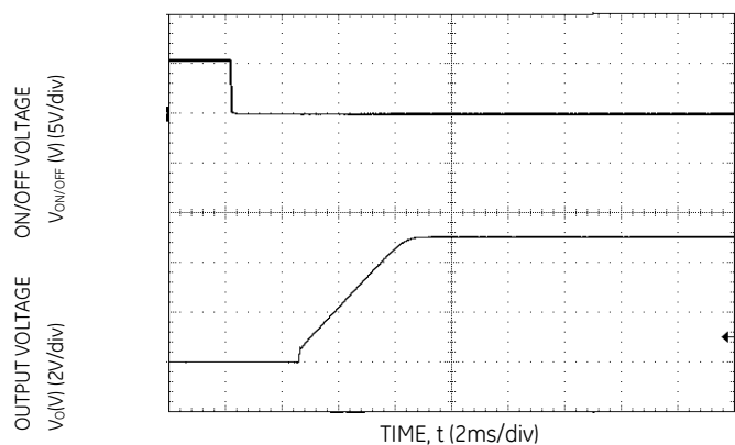
Figure 35. Typical Start-up Using On/Off Voltage ( I_o = I_{o,max} ).
