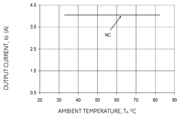
Figure 31. Derating Output Current versus Ambient Temperature and Airflow.
