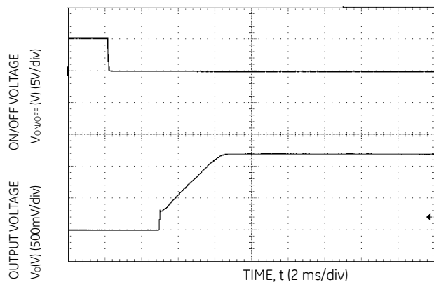
Figure 11. Typical Start-up Using On/Off Voltage ( I_o = I_{o,max} , V_{IN} = 8V ).
