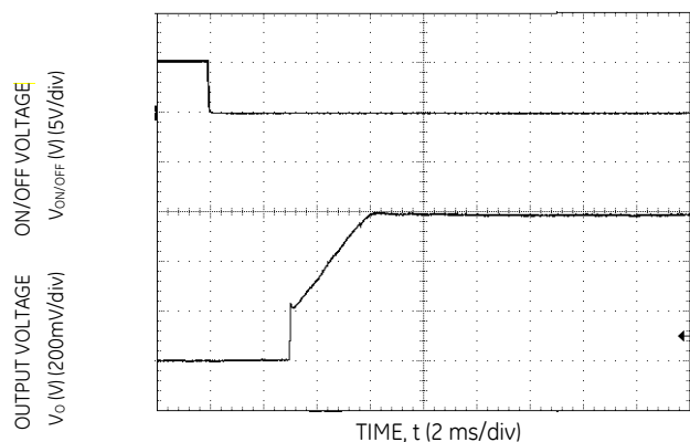
Figure 5. Typical Start-up Using On/Off Voltage ( I_o = I_{o,max} , V_{IN} = 8V )
