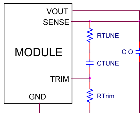
Figure 59. Circuit diagram showing connection of R_{TUNE} and C_{TUNE} to tune the control loop of the module.
