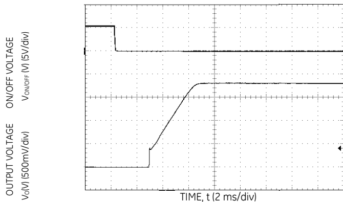
Figure 17. Typical Start-up Using On/Off Voltage ( I_o = I_{o,max} ).
