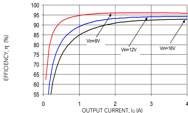
Figure 37. Converter Efficiency versus Output Current.
