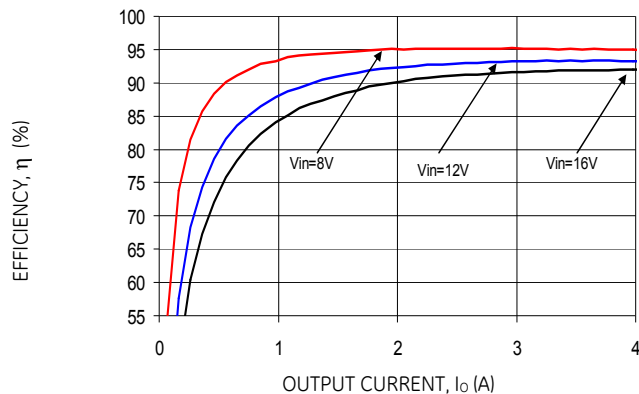
Figure 31. Converter Efficiency versus Output Current.
