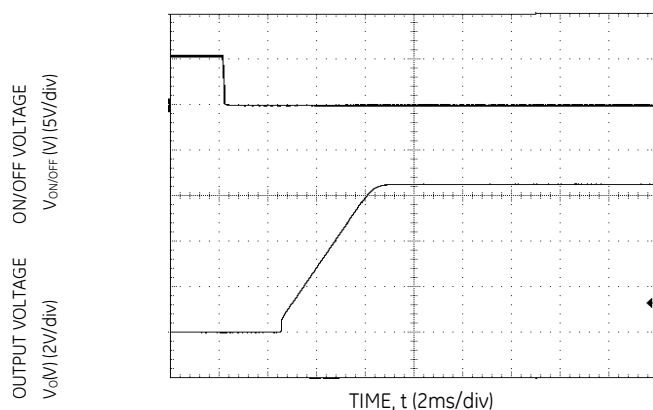
Figure 41. Typical Start-up Using On/Off Voltage ( I_o = I_{o,max} ).
