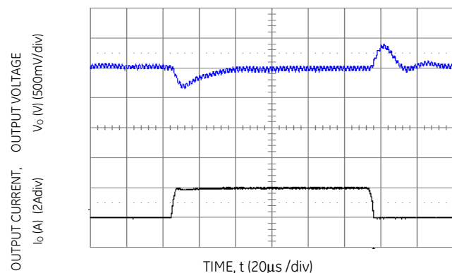
Figure 34. Transient Response to Dynamic Load Change from 0% 50% to 0%.
