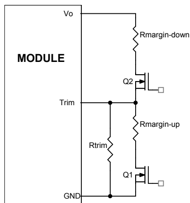
Figure 58. Circuit Configuration for margining Output voltage.
